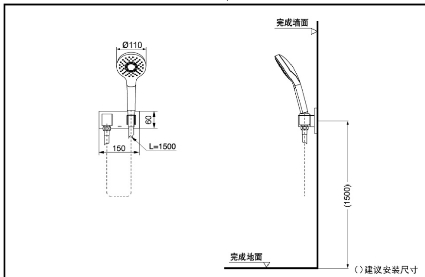
TBW01008B3 Wall-Mounted Handshower
