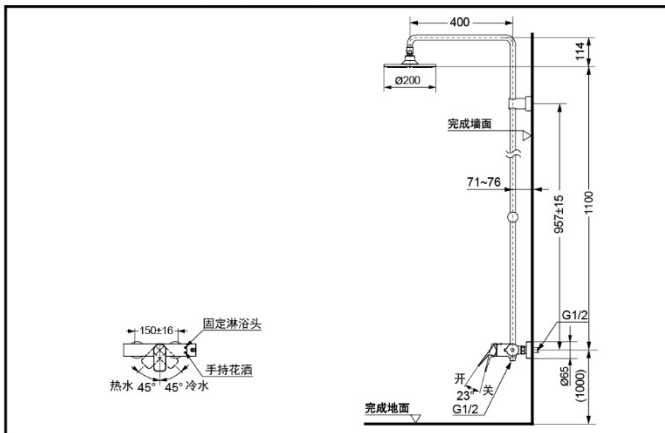
DM919CAR Shower Bar
