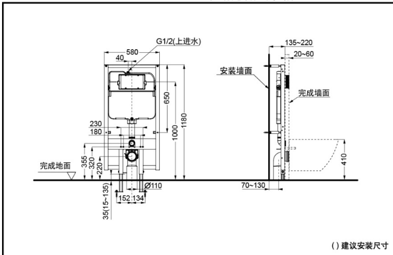
WH172B-162B/WH172B-762B 手动隐藏式水箱
