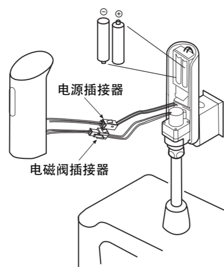
DUE110PBK*/DUE110PSK*/DUE138PSK*
