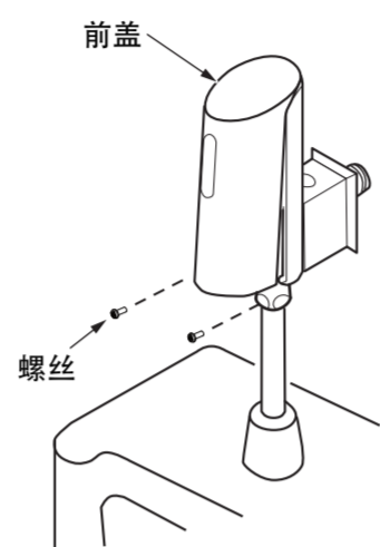
DUE110PBK*/DUE110PSK*/DUE138PSK*
